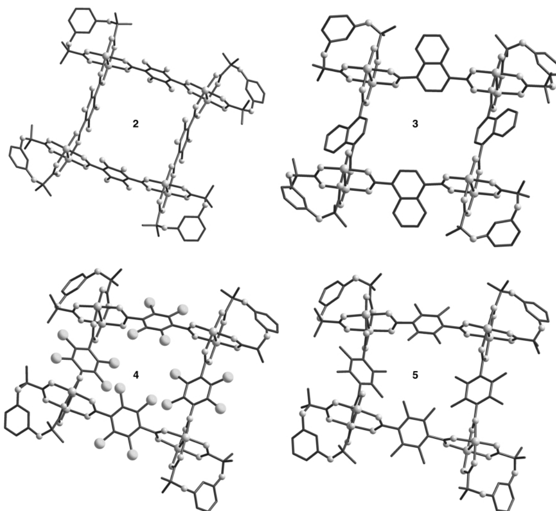
Fig. 1 Crystal structures of 2–5 (axial ligands, solvent molecules and hydrogens omitted). The dirhodium corners are spaced 10.9–11 Å apart. The Rh–Rh bonds (2.37–2.39 Å), Rh–O bonds to the axial oxygen ligands (2.24–2.34 Å) and the Rh–O bonds in the Rh–O cages (2.01–2.06 Å) are in the normal range for dirhodium tetracarboxylates. 10
