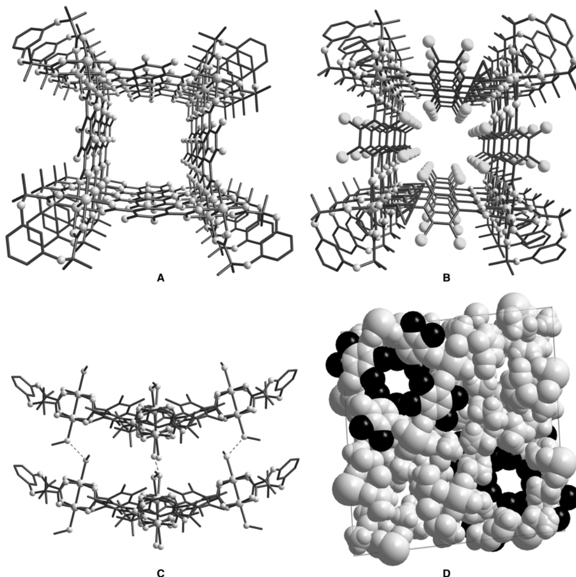
Fig. 2 (A) Offset stacking of 2 , looking down the channel. (B) Vertical stacking of 4 . Box 5 packs in a similar fashion. (C) Two molecules in a stack of 5 , viewed across the box diagonal, showing the saddle distortion of the framework and hydrogen bonds connecting axially coordinated methanol and water ligands. (D) Space filling view of the unit cell of 4 , with chlorines in black, all other atoms light grey.
