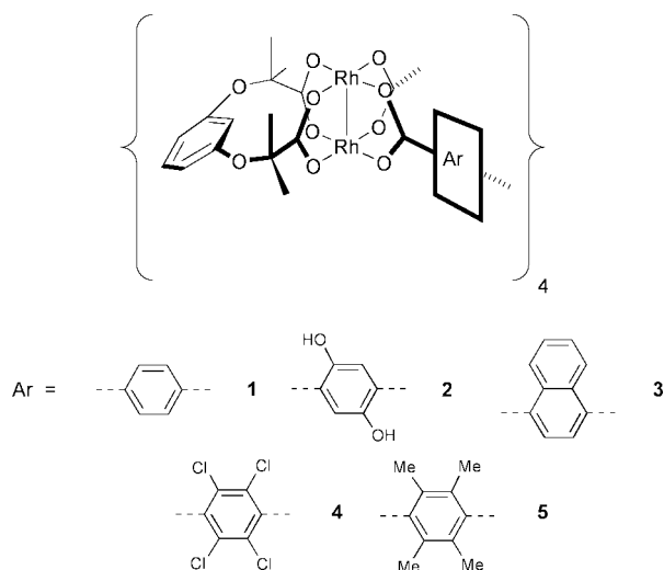
Fig. 2 (A) Offset stacking of 2 , looking down the channel. (B) Vertical stacking of 4 . Box 5 packs in a similar fashion. (C) Two molecules in a stack of 5 , viewed across the box diagonal, showing the saddle distortion of the framework and hydrogen bonds connecting axially coordinated methanol and water ligands. (D) Space filling view of the unit cell of 4 , with chlorines in black, all other atoms light grey.
